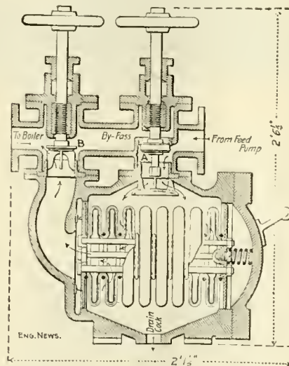
FIG. 2.—ROSS FEED-WATER FILTER.
